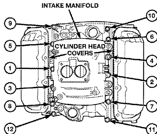
FRONT OF ENGINE 3.9L Intake Manifold Bolt Tightening Sequence
